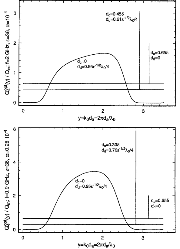
Figure 2: Optimum Q ( N=4 ) of metalodielectric filters for normal plane-wave incidence.
